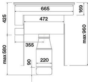
Frontal view
