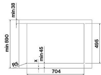
Hole dimensions
