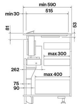
Side view with motor in front position
