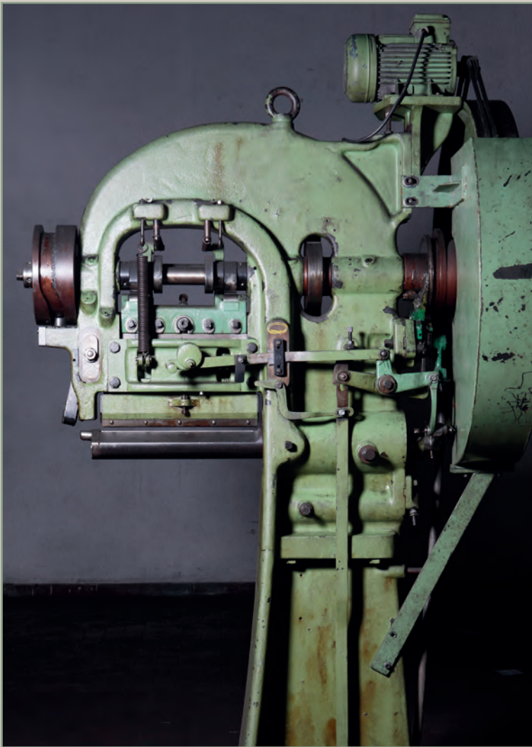
From the company's historical archive: machine for stitching sheet metal, 1950s.
