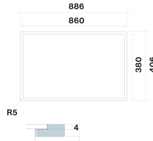
Flush installation
